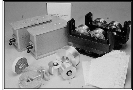
B5F Kit of Parts, typical
